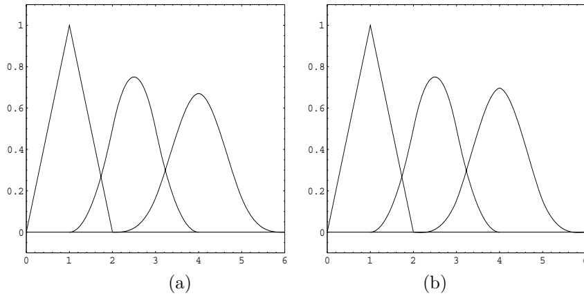
Fig. 1. The discrete GB-splines B_{j,k} , k = 2, 3, 4 (from left to right) on a uniform mesh with step size h_i = 1 , no tension and discretization parameter \tau = 0.1 (a) and \tau = 0.33 (b).
