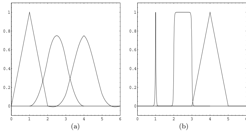
Fig. 2. Same as Figure 1, but with discretization parameter \tau = 0.5 (a) and with tension parameters q_i = 50 , for all i (b).
