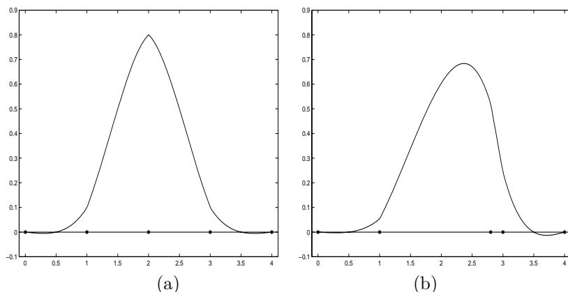
Fig. 3. The discrete GB-splines B_{j,4} on a uniform mesh (a) and on a non-uniform mesh (b). The asterisk * denotes the x_i . For both plots q_i = 2 and \tau = 0.5 .
